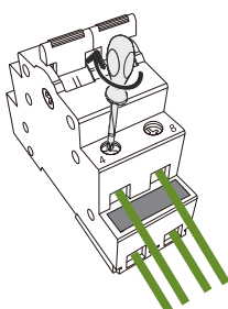
4 Wiring on top and tightening the screws
