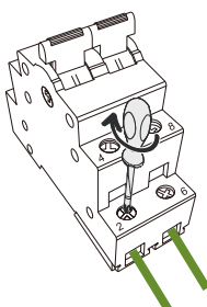
2 Tighten the screws
